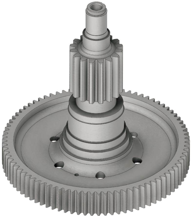
PLANET GEAR ASSEMBLY
